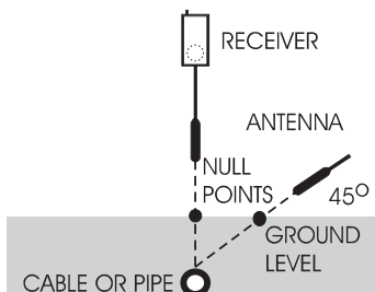
Fig. 02 - Measuring Depth
